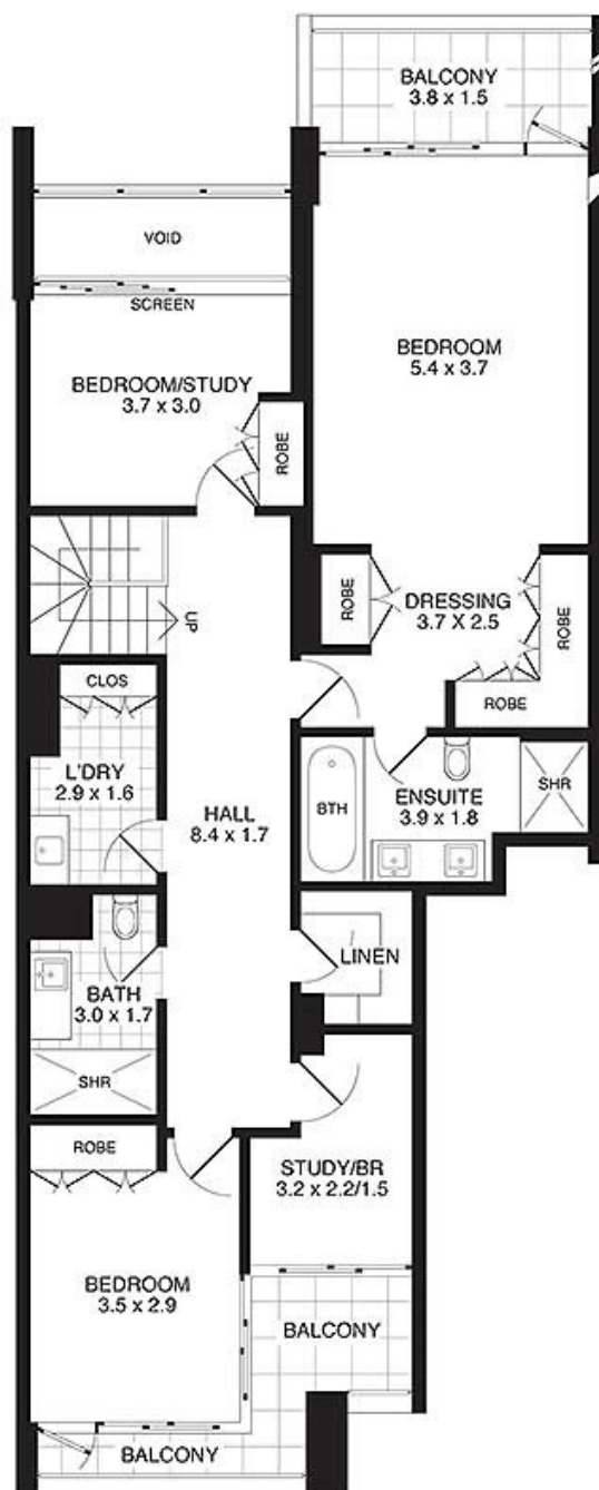
LEVEL 2 Scale 1cm = 1m (approx)
