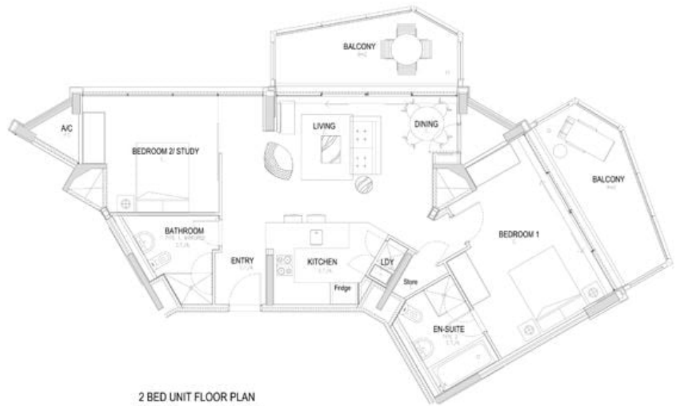
2 BED UNIT FLOOR PLAN Scale: 1/50 Floor Area 87m 2 APARTMENT PLAN
